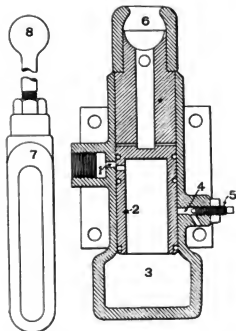
Figs. 3261-3262. Simplicity Bell Ringer. Adreon & Co.
